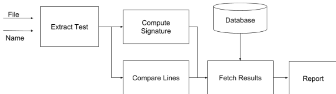
Figure 2. Workflow Diagram
